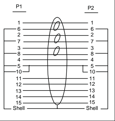
PIN Assignment
